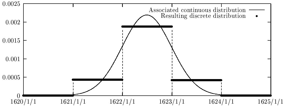
Figure 1. The STRICTLY_AROUND distribution.
